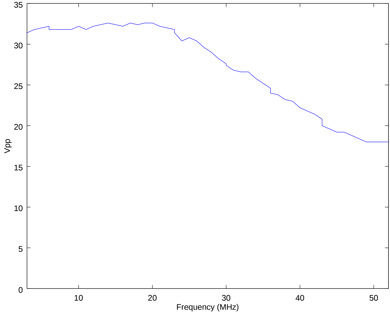
Si5351a Linearity Test
