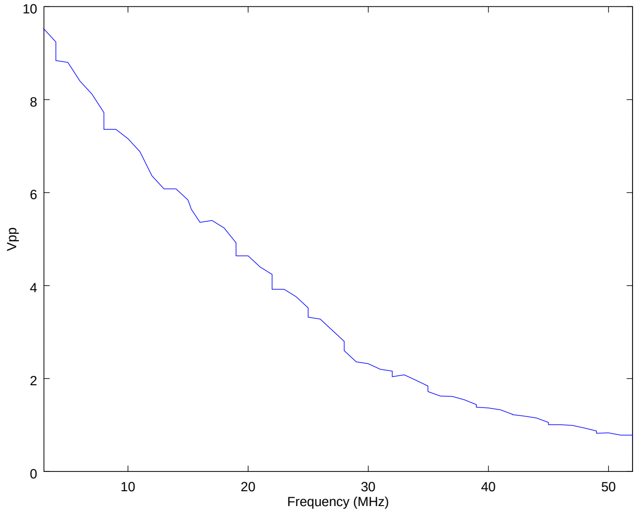
AD9851 Linearity Test
